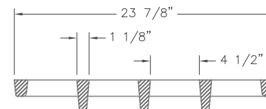
TYPICAL GRATE SECTION
