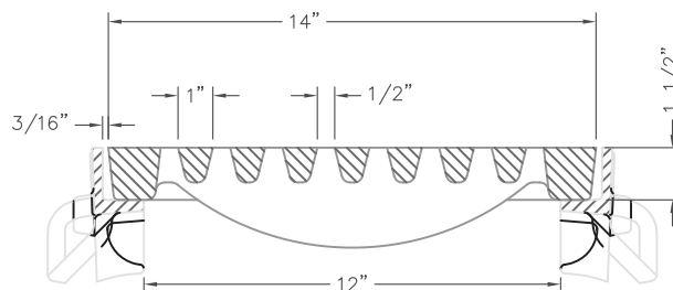
R-4990-DX TYPE "Q" GRATE w/ TYPE "B" FRAME TYPICAL SECTION (SCALE: 1/4"=1")
